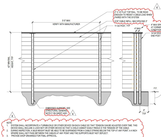
1 AGS PREFABRICATED SS CABLE RAILING RAINIER DETAIL 1" = 1'-0"
