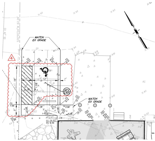
GRADING ENLARGEMENT A 1" = 8'
