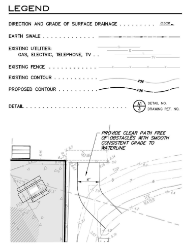
GRADING ENLARGEMENT B 1" = 8'
