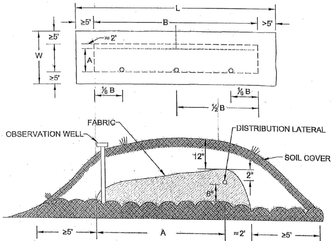
PLAN VIEW AND CROSS SECTION OF WISCONSIN AT-GRADE UNIT WITH A SINGLE ABSORPTION AREA ON A SLOPING SITE
