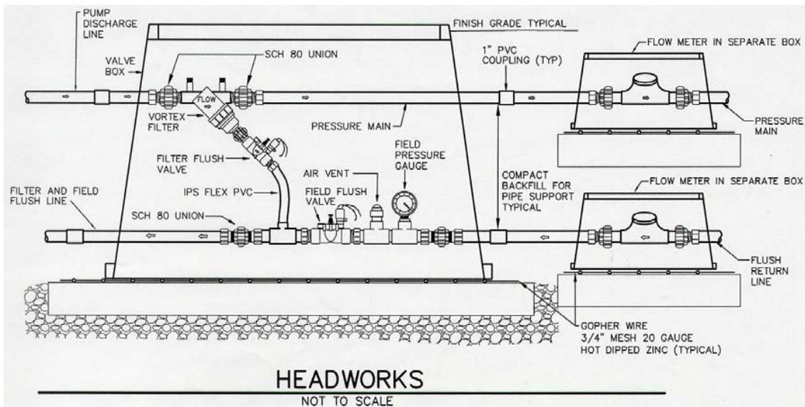
Figure 13.7f – Headworks
