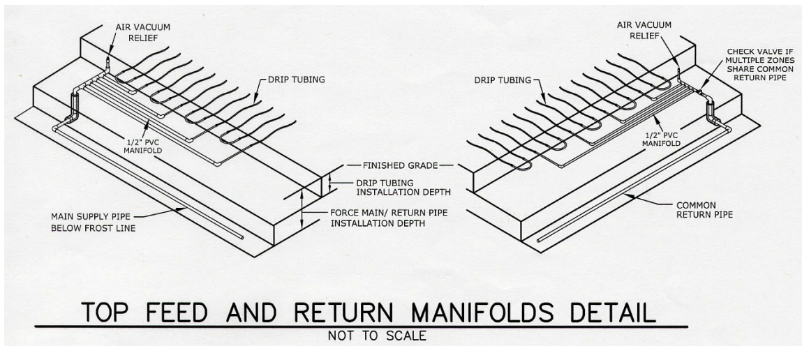
Figure 13.7d Manifold Connection
