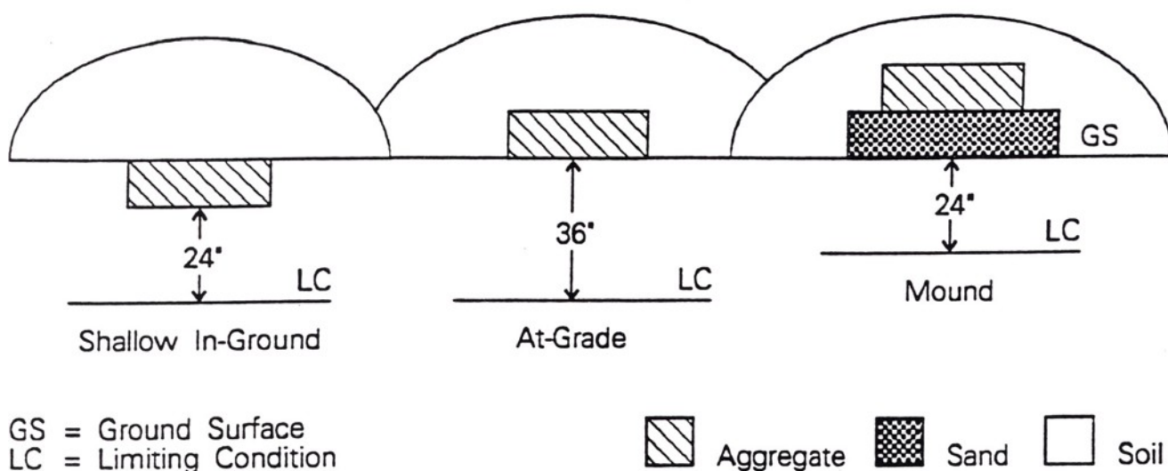
Figure 13.5a SIG (requires pretreatment), At-Grade, Mound Soil Below Trench Bottom Requirements
