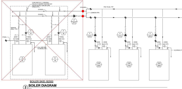
5. EXISTING BOILER PIPING DIAGRAM SCALE: 1/8"
