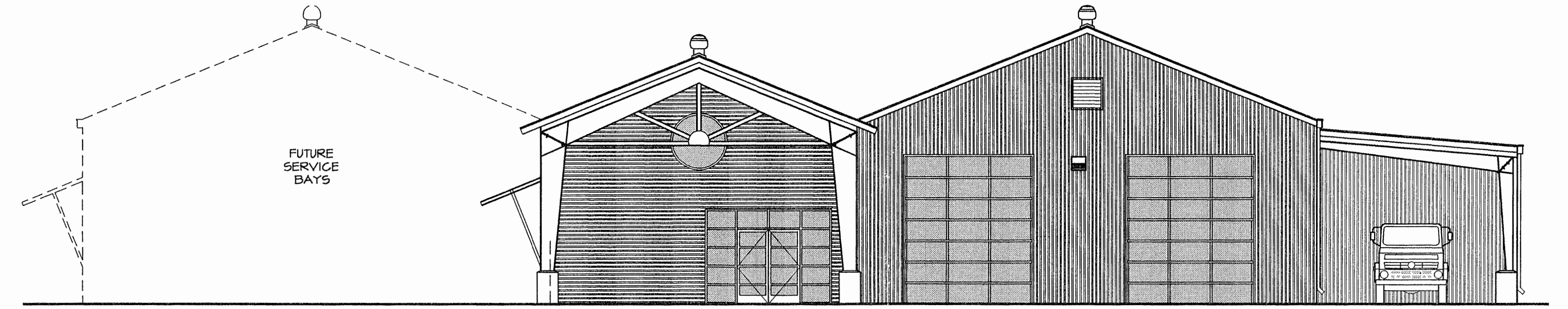
SOUTH ELEVATION
