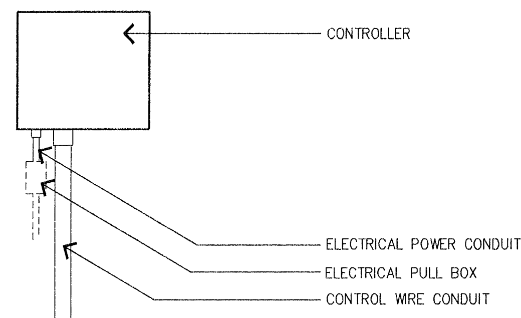
WALL MOUNT CONTROLLER
