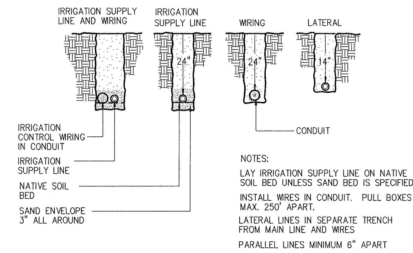
TRENCHING AND INSTALLATION
