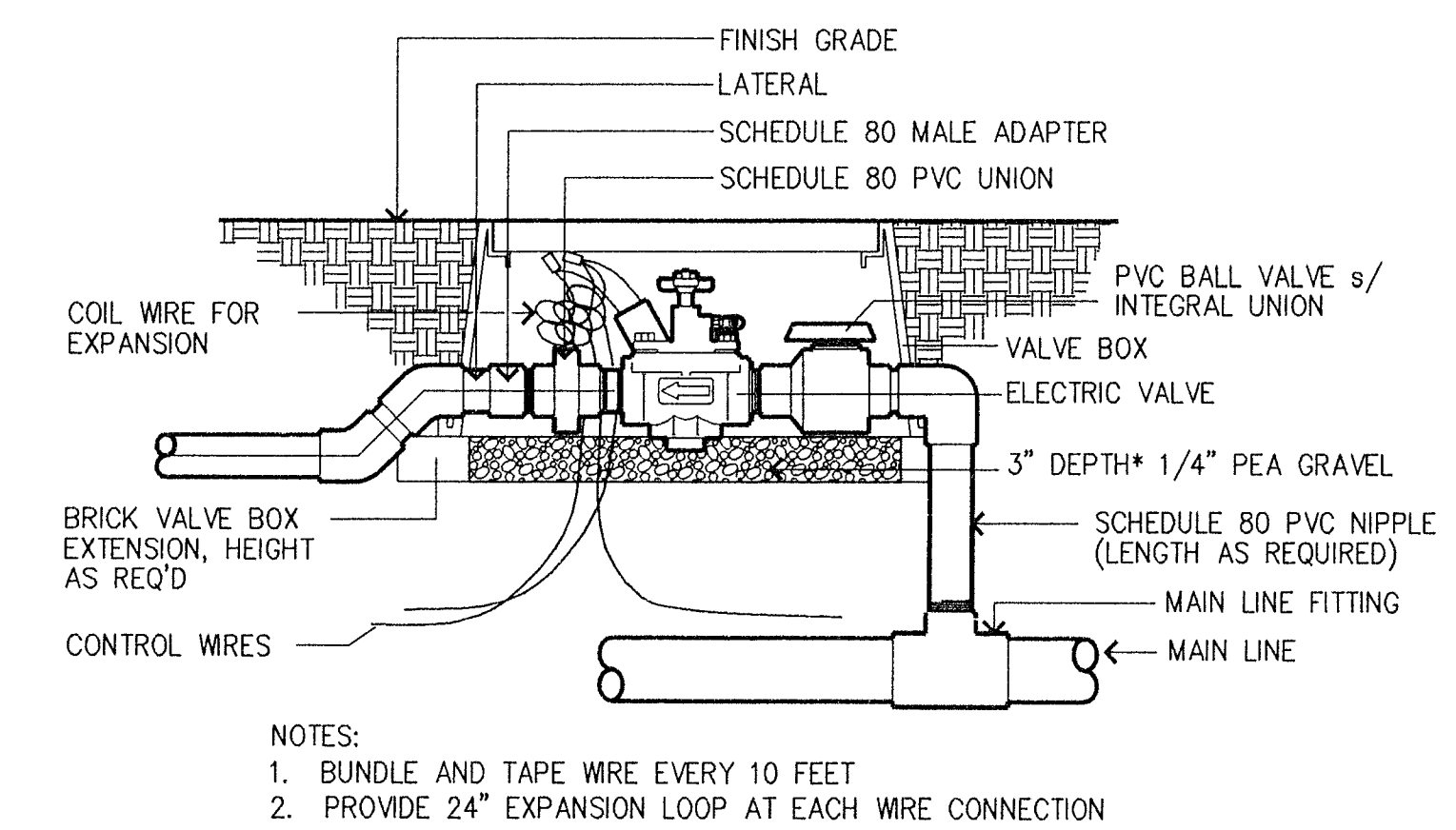
REMOTE CONTROL VALVE
