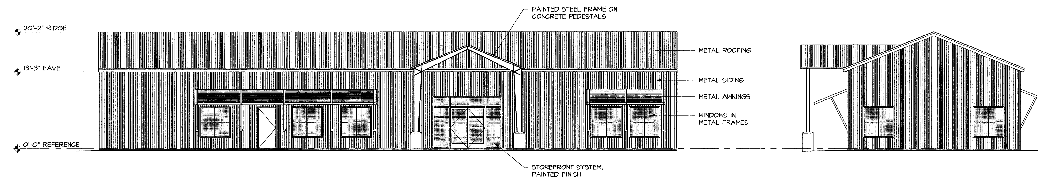
EAST ELEVATION
