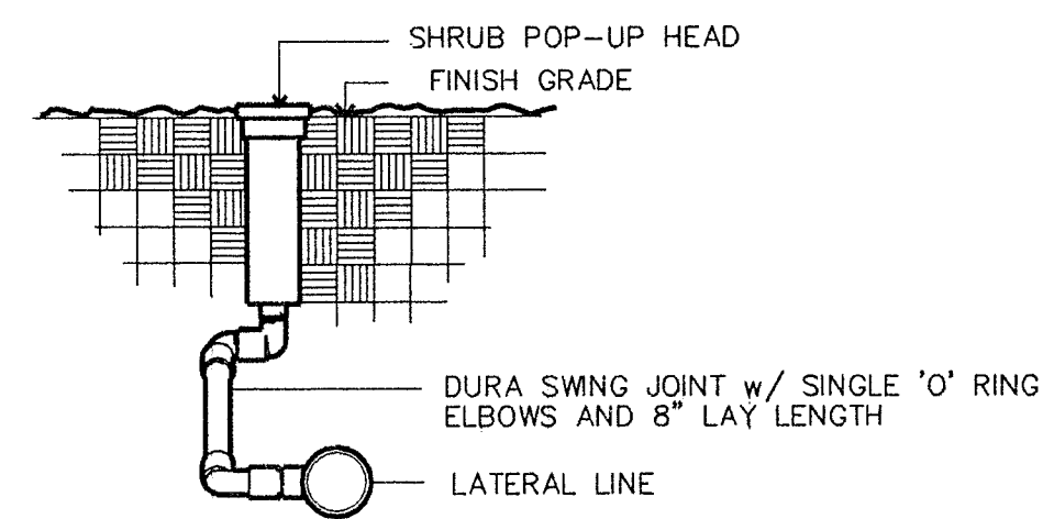
SHRUB POP-UP SPRAY HEAD
