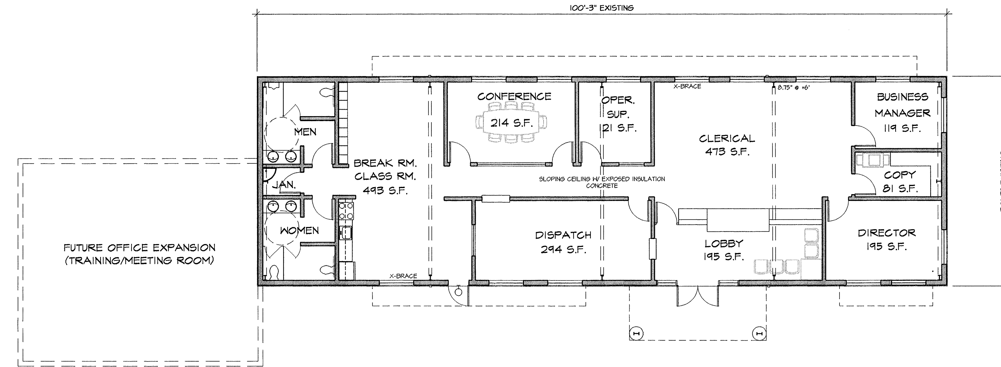
FLOOR PLAN
