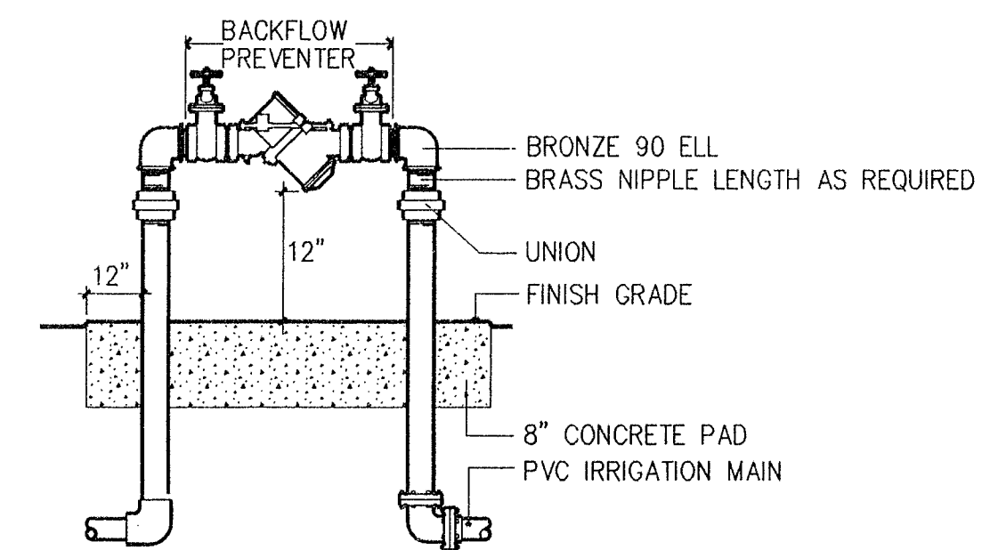
REDUCED PRESSURE BACKFLOW PREVENTER
