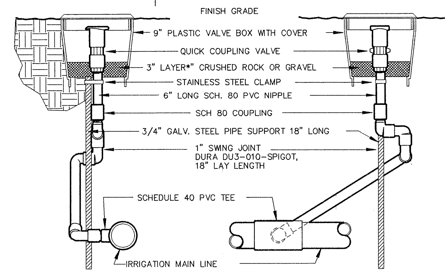
QUICK COUPLING VALVE
