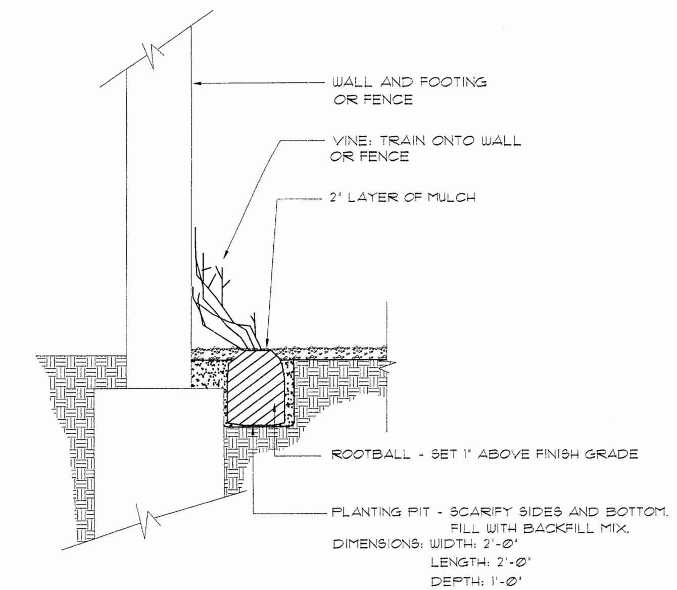
3 VINE PLANTING DETAIL NOT TO SCALE
