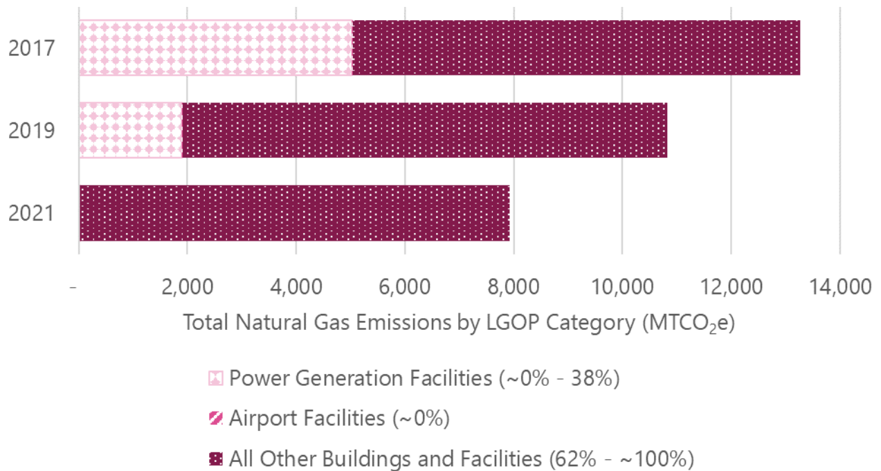
Figure 17. Natural gas emissions by LGOP category (MTCO 2e ).
