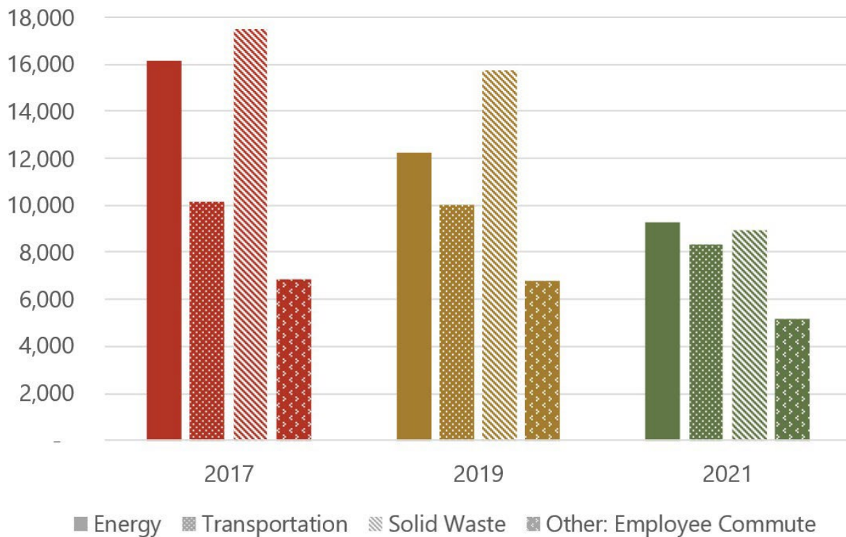
Figure 9. GHG emissions by source for 2017, 2019 and 2021.
