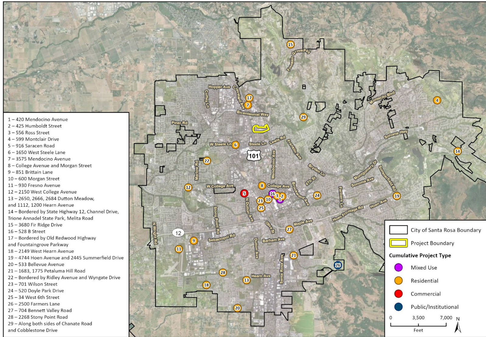
Figure 3-1 Cumulative Projects
