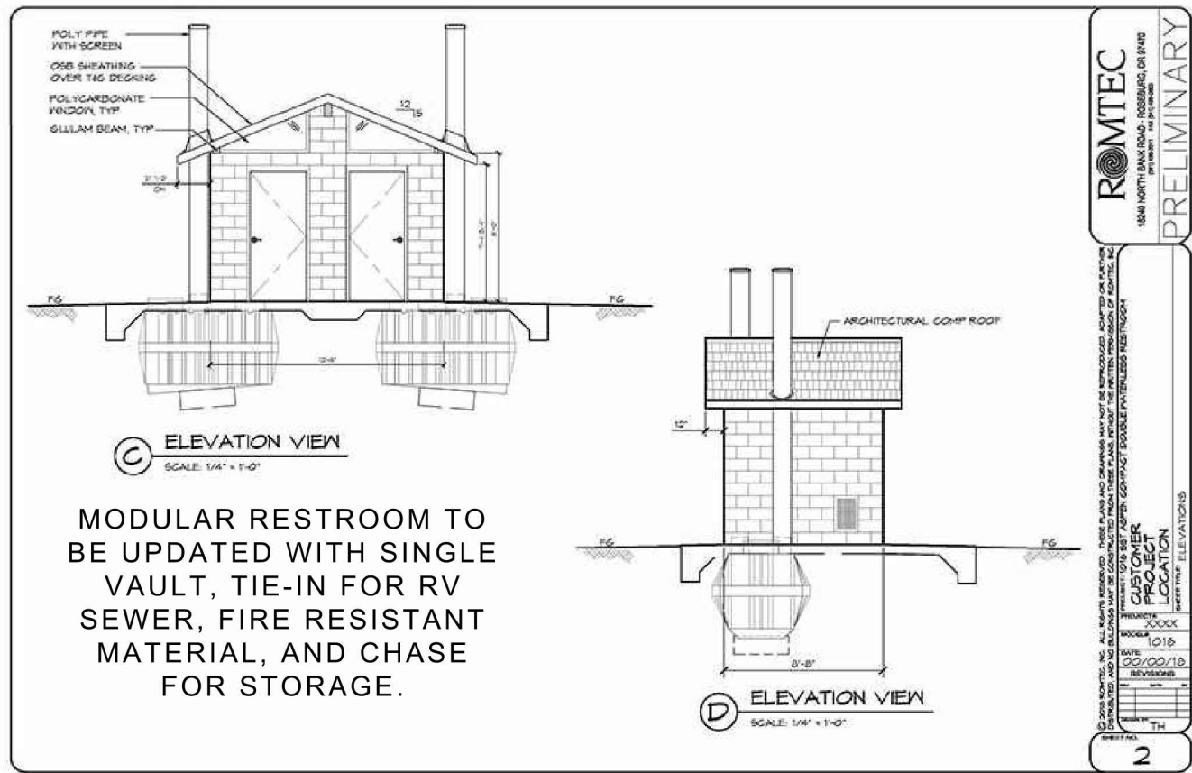
MODULAR FLOOD-PROOF VAULT BATHROOM EXAMPLE BY ROMTEC
