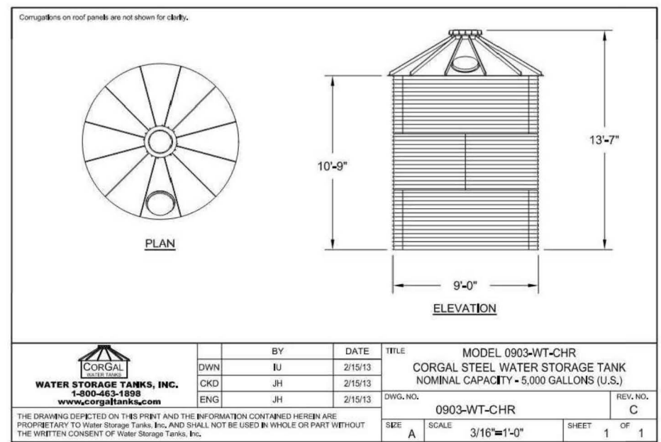
FIRE RESISTANT WATER STORAGE TANK EXAMPLE
