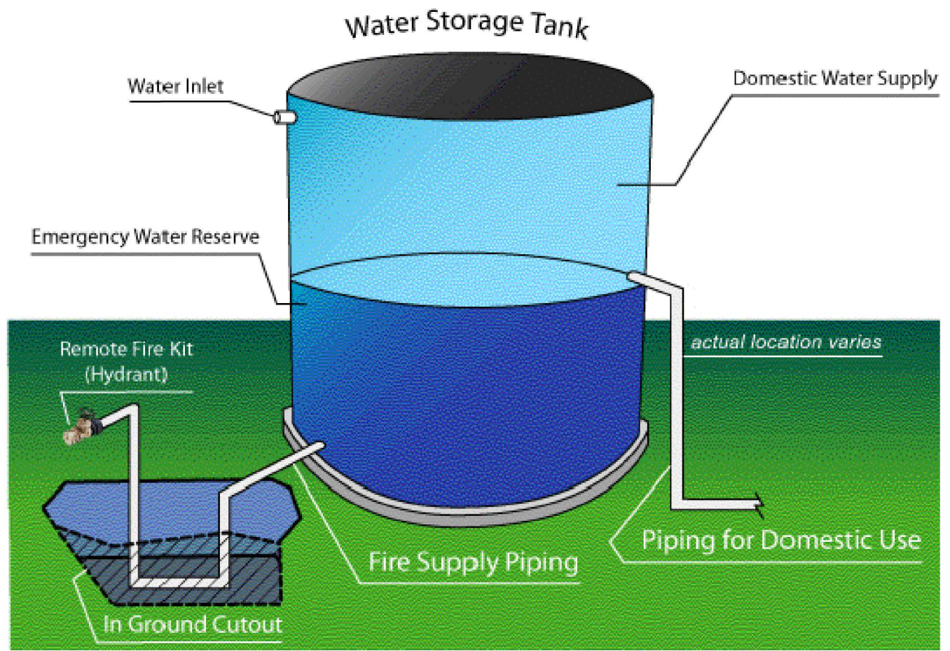
DIAGRAM OF WATER RESERVE SYSTEM FOR FIRE SUPPRESSION
