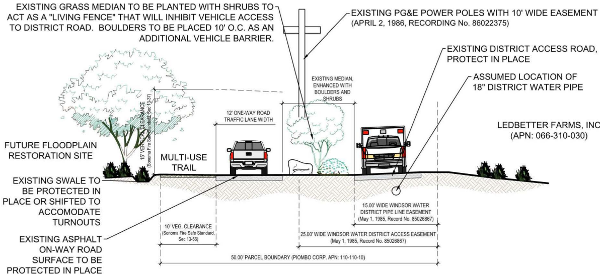
1 NORTH ONE-WAY ROAD ACCESS - TYPICAL CROSS SECTION
