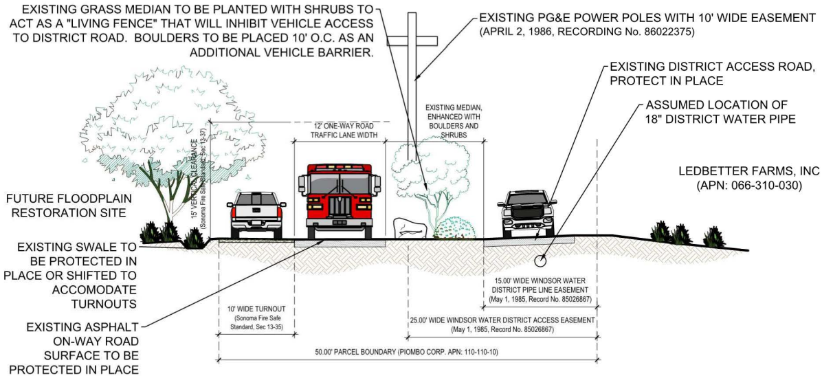
2 NORTH ONE-WAY ROAD TURNOUT - TYPICAL CROSS SECTION
